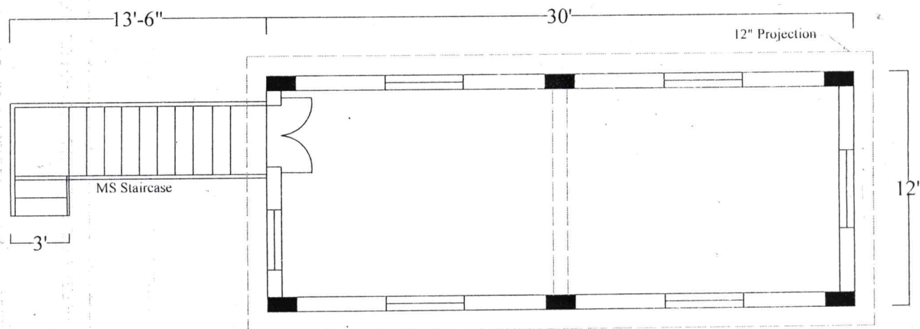
LAYOUT PLAN
