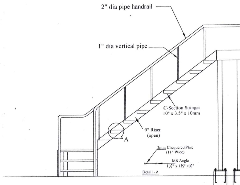
L-Shaped MS Staircase Detail
